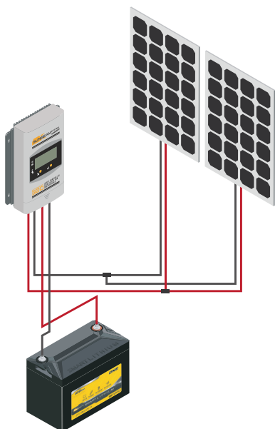
PARALLEL CONNECTION
