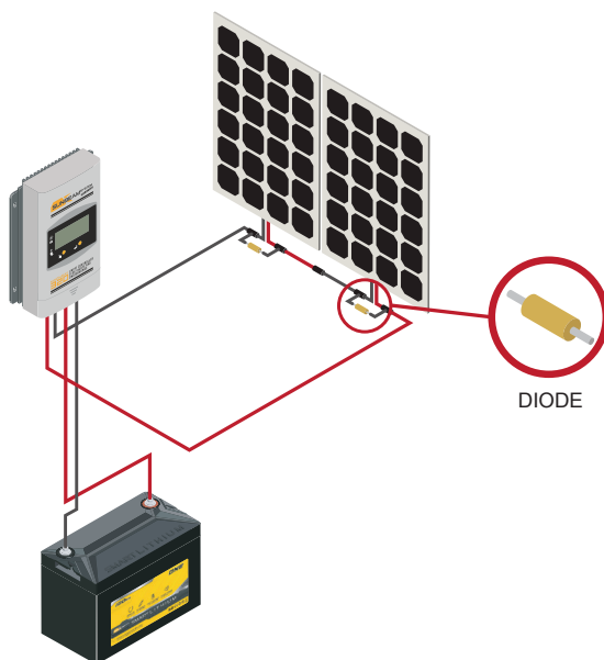
SERIAL CONNECTION
